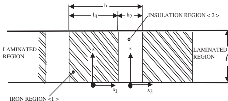
Figure 1. Laminated structure.
